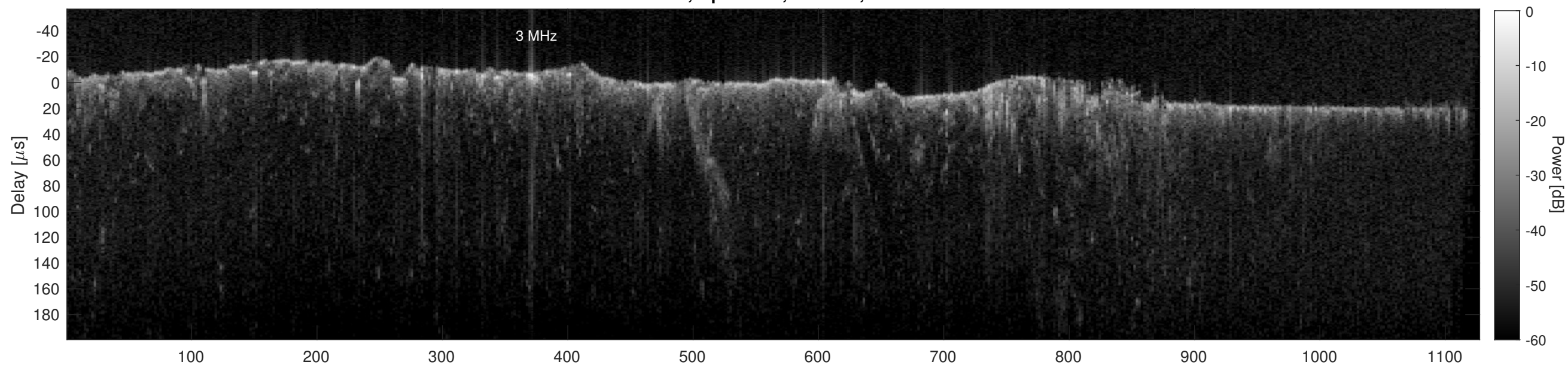
Orbit 12285, Cluttergram
