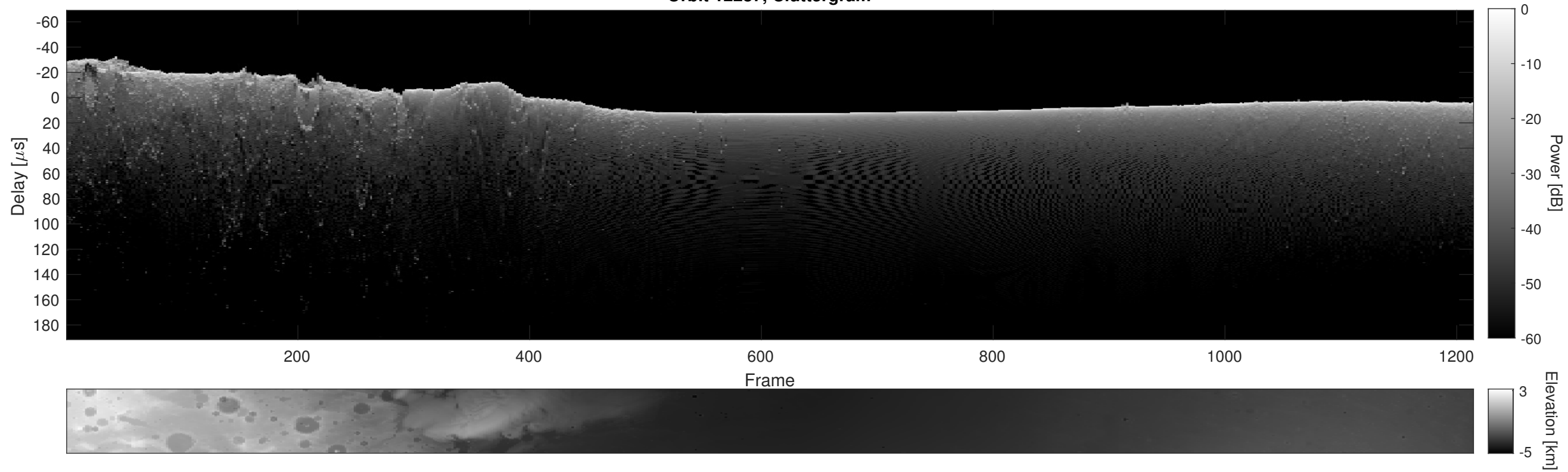
Orbit 12287, Cluttergram
