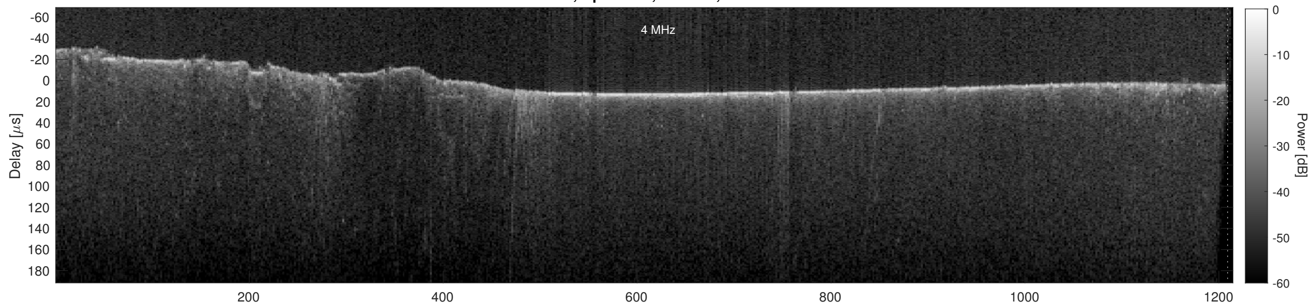
Orbit 12287, Cluttergram
