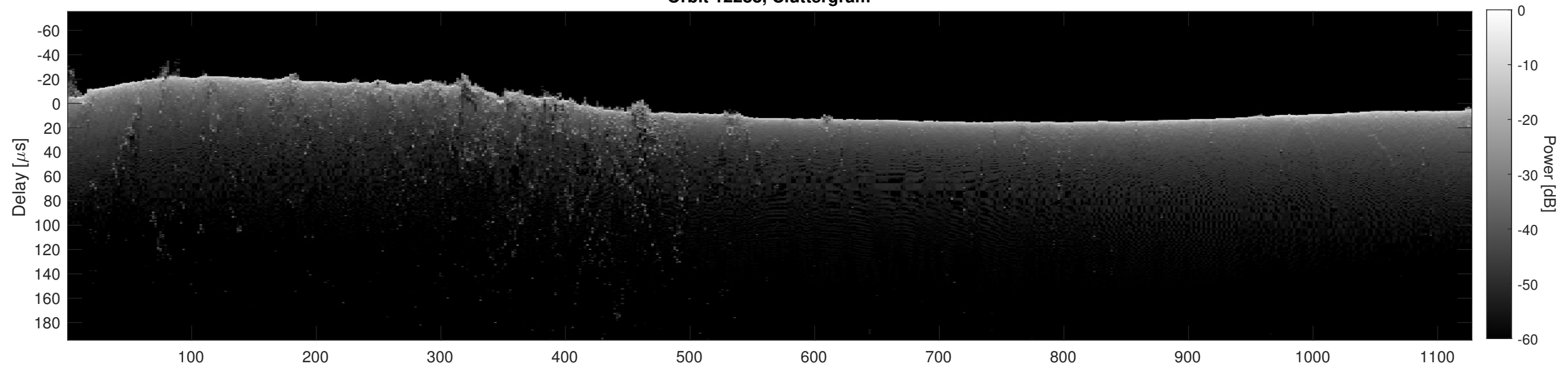
Orbit 12288, Cluttergram
