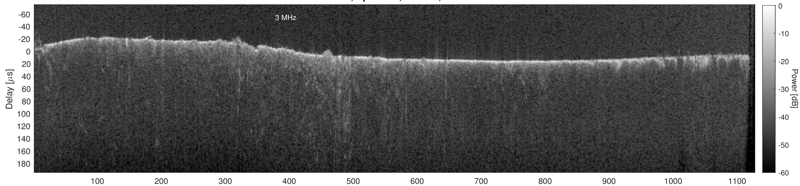
Orbit 12288, Cluttergram
