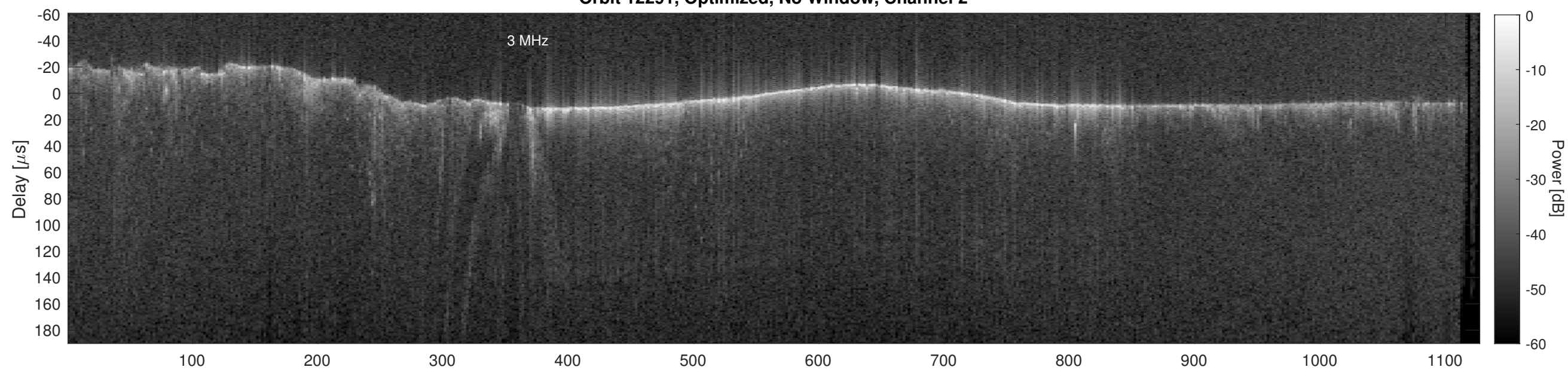
Orbit 12291, Cluttergram
