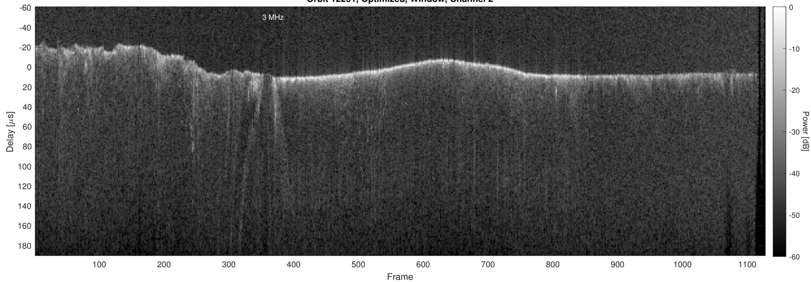
Orbit 12291, Optimized, Window, Channel 2
