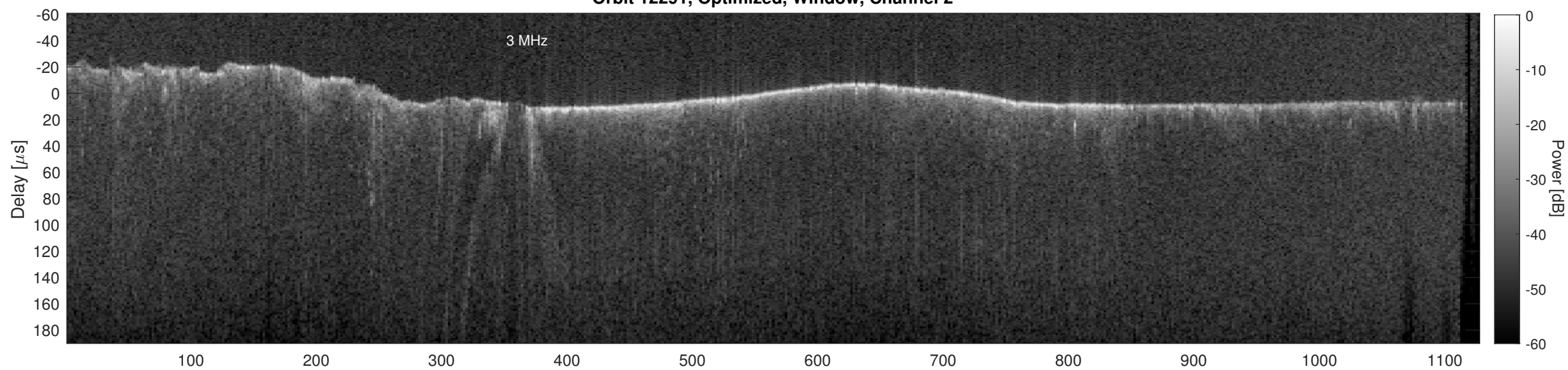
Orbit 12291, Cluttergram
