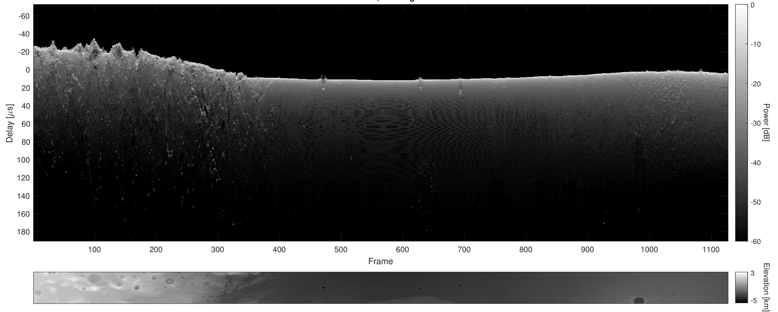
Orbit 12294, Cluttergram
