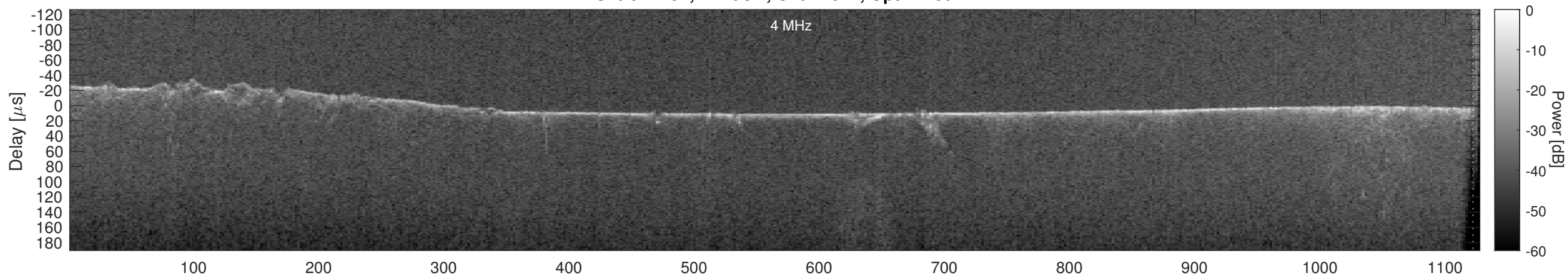
Orbit 12294, Cluttergram
