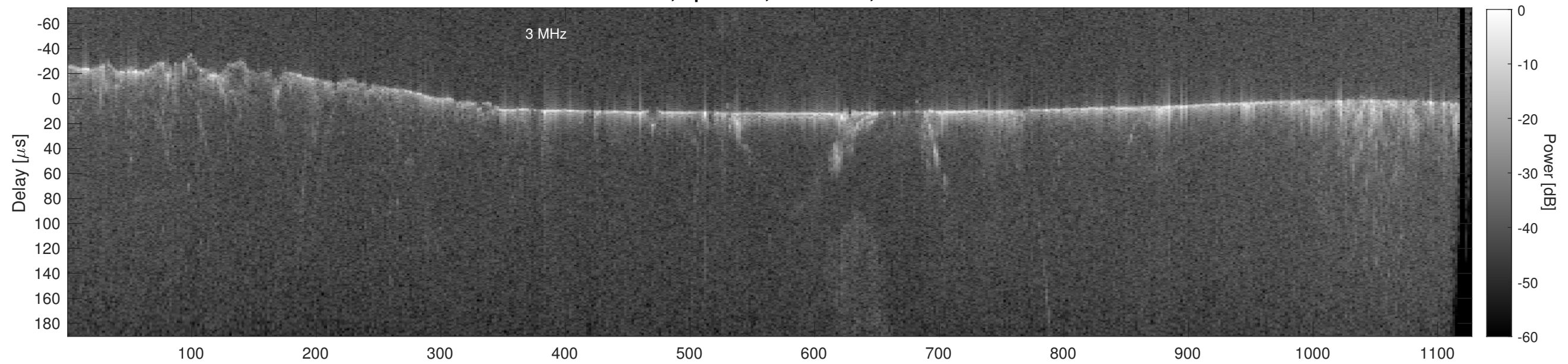
Orbit 12294, Cluttergram
