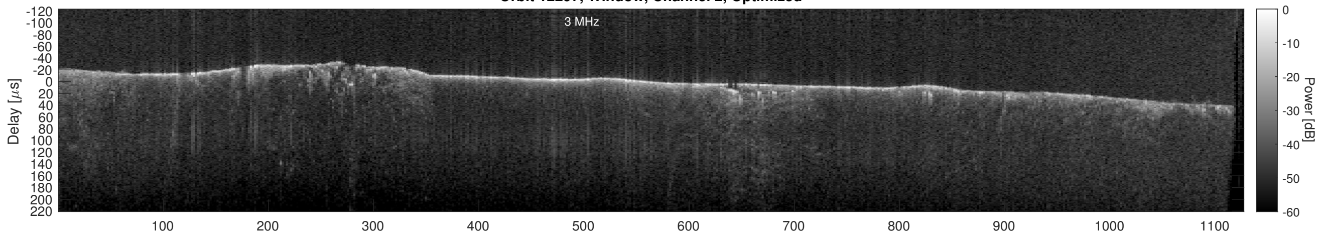
Orbit 12297, Cluttergram
