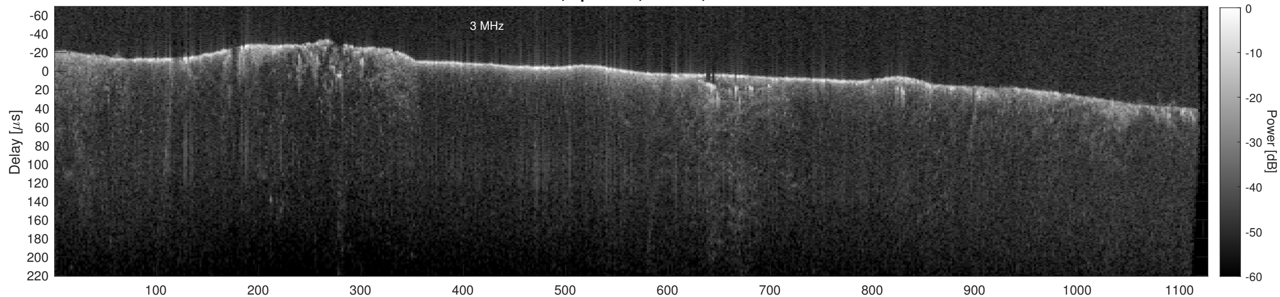
Orbit 12297, Cluttergram
