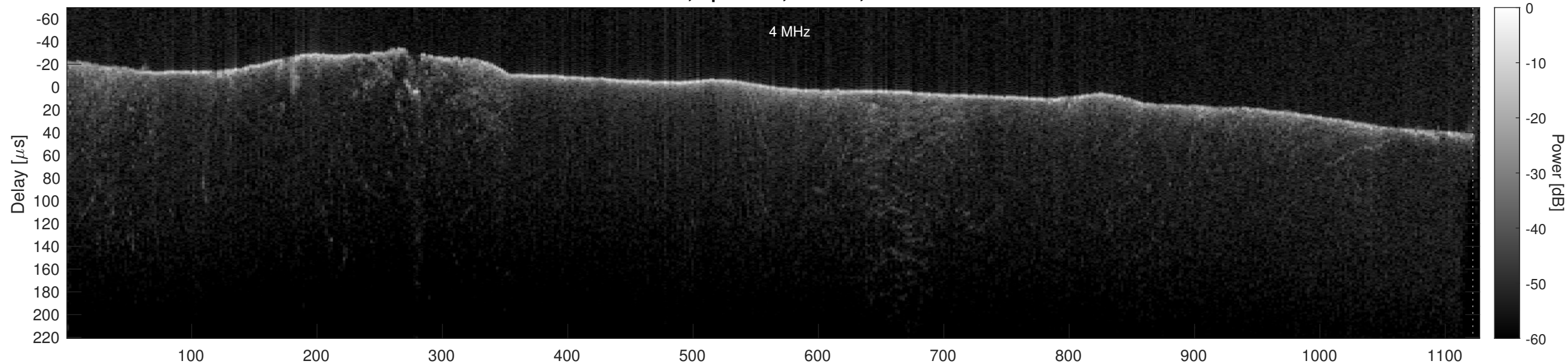
Orbit 12297, Optimized, Window, Channel 2
