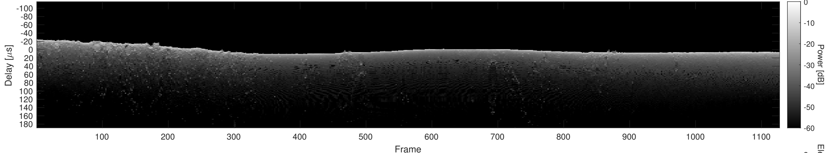
Orbit 12298, Cluttergram
