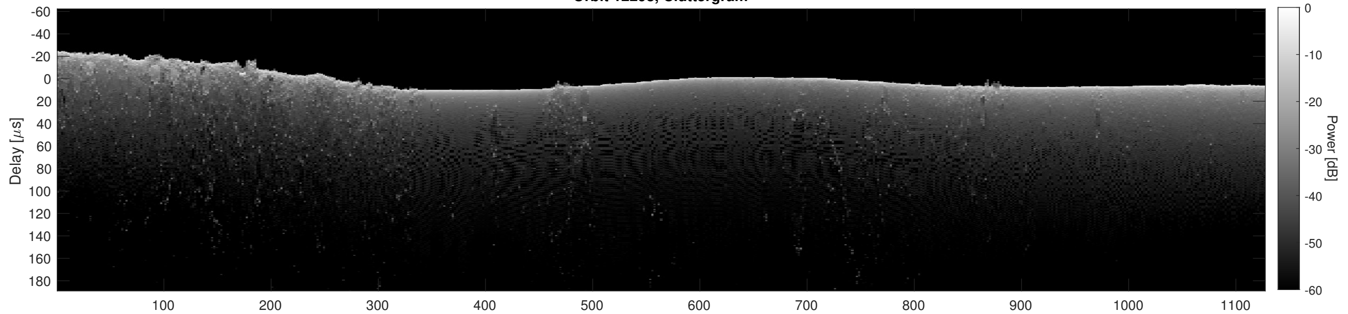
Orbit 12298, Cluttergram
