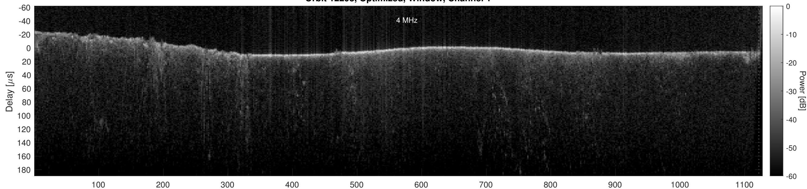
Orbit 12298, Optimized, Window, Channel 2
