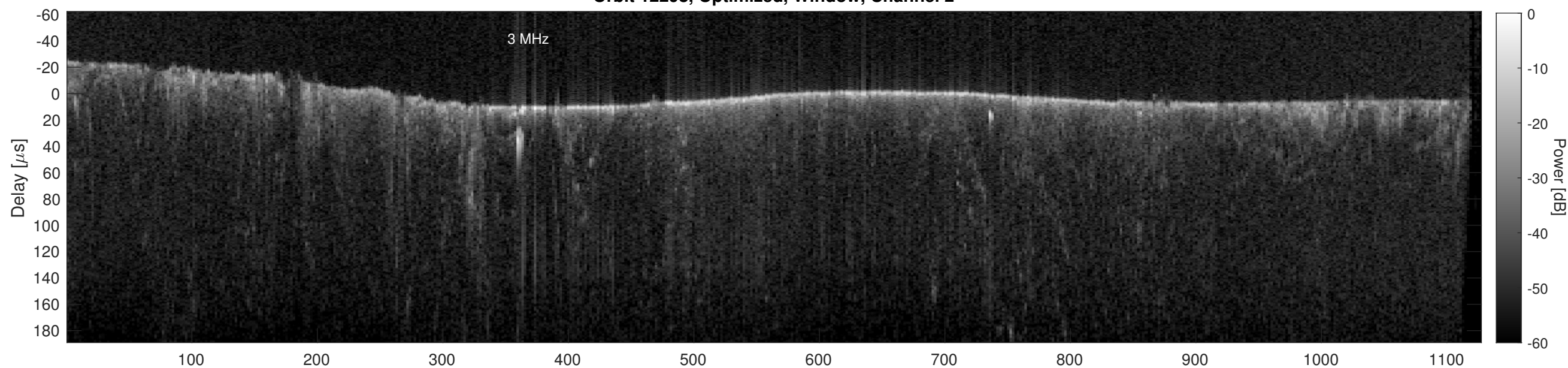
Orbit 12298, Cluttergram
