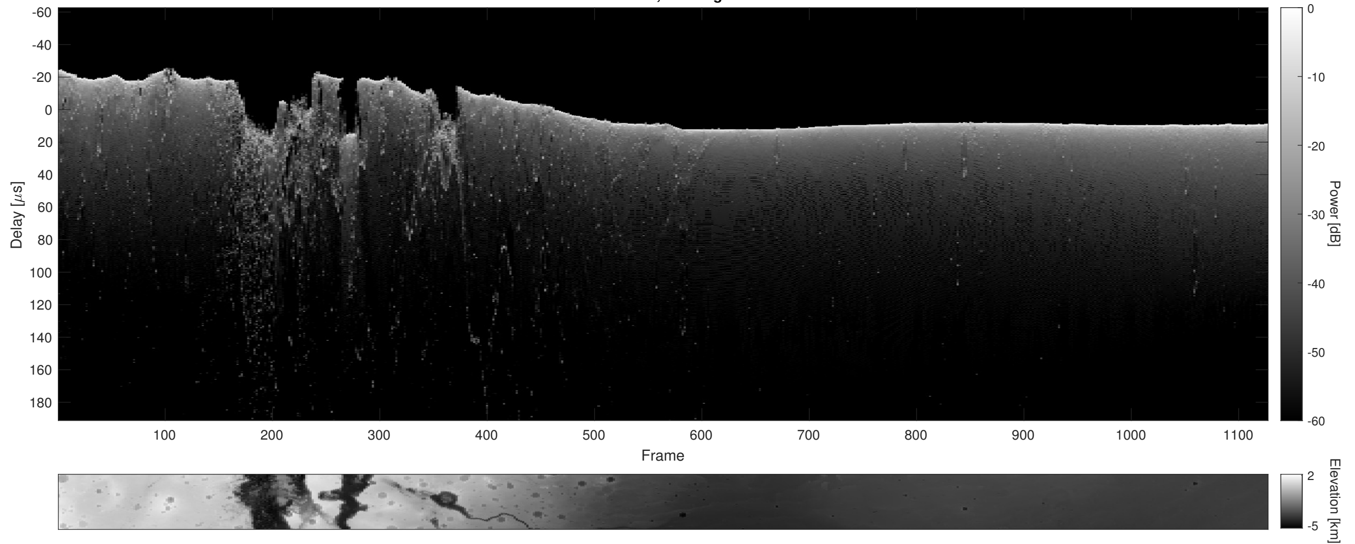
Orbit 12300, Cluttergram
