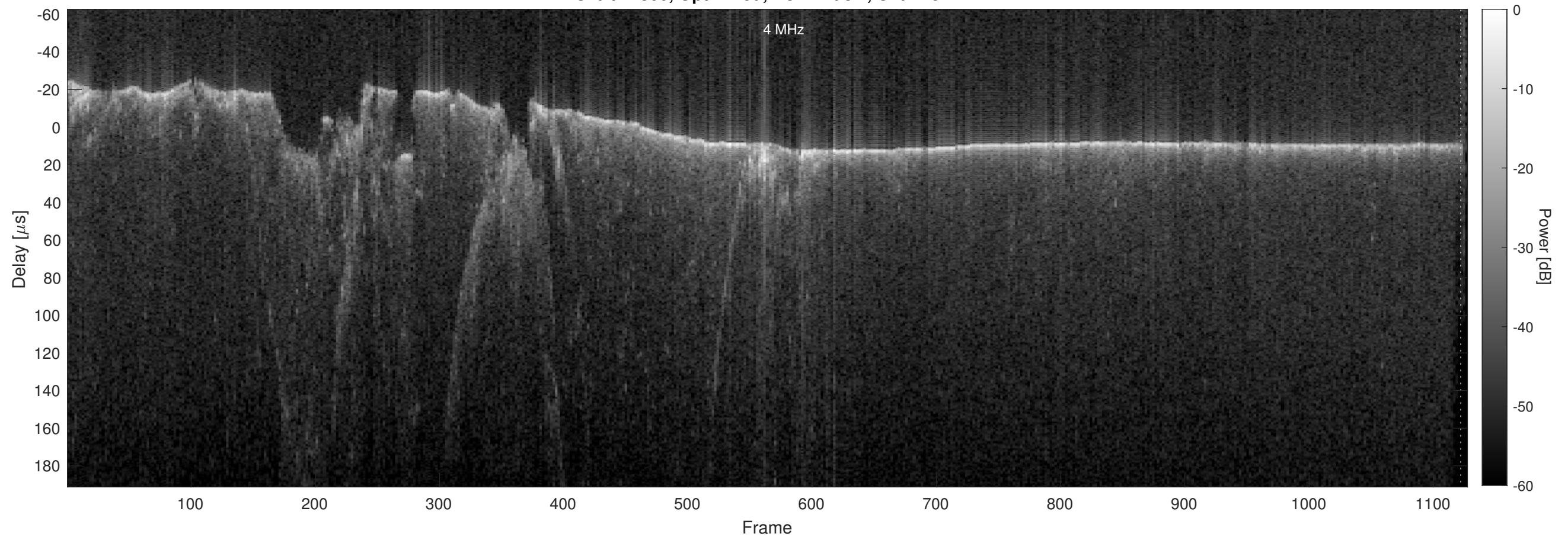
Orbit 12300, Optimized, No Window, Channel 2
