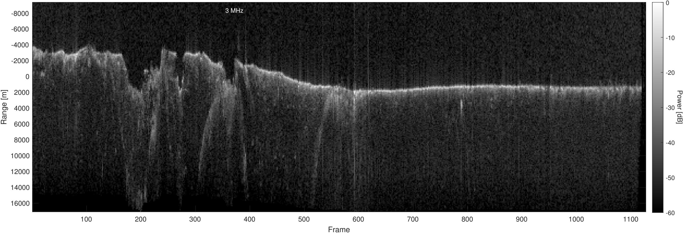
Orbit 12300, Optimized, Window, Depth-Corrected, Channel 2
