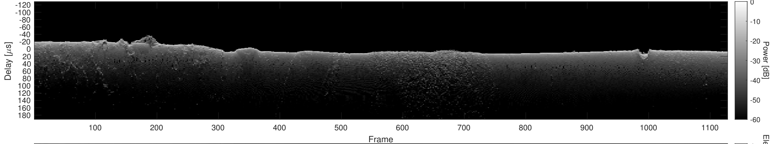
Orbit 12301, Cluttergram
