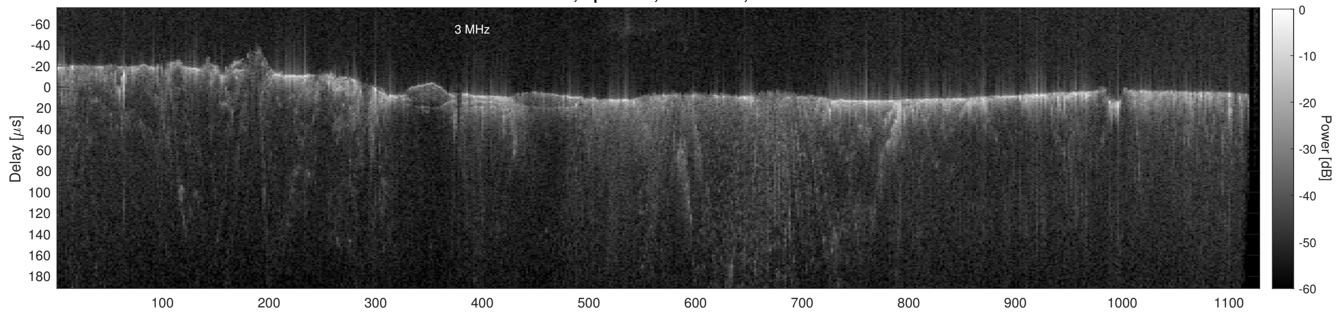
Orbit 12301, Cluttergram
