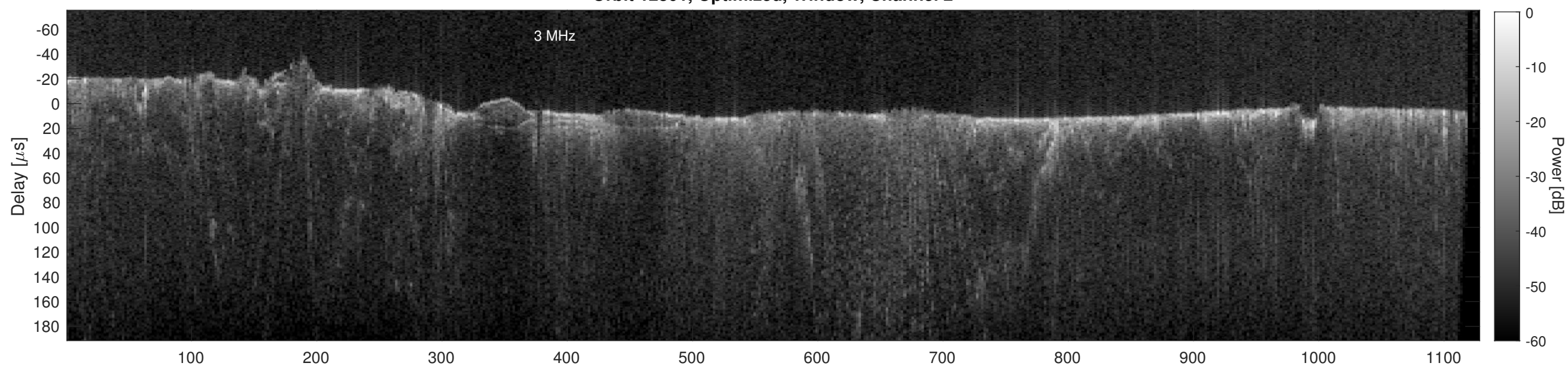
Orbit 12301, Cluttergram
