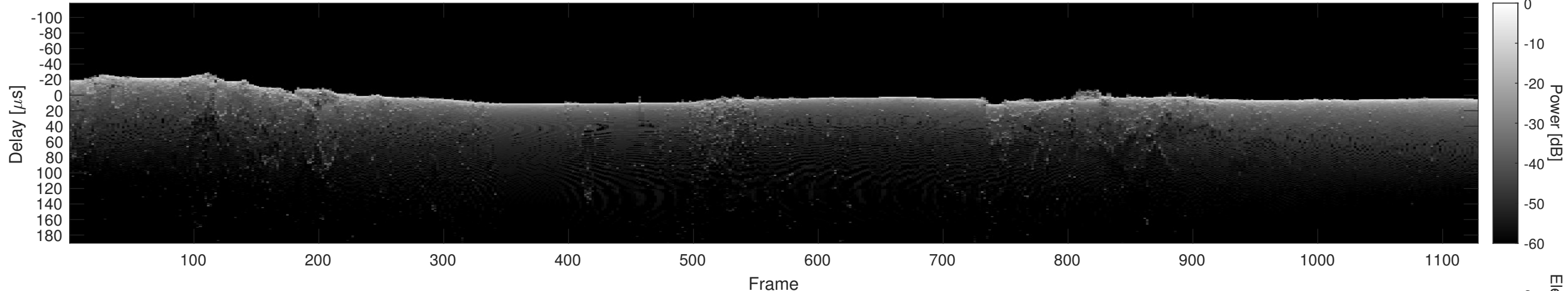
Orbit 12305, Cluttergram
