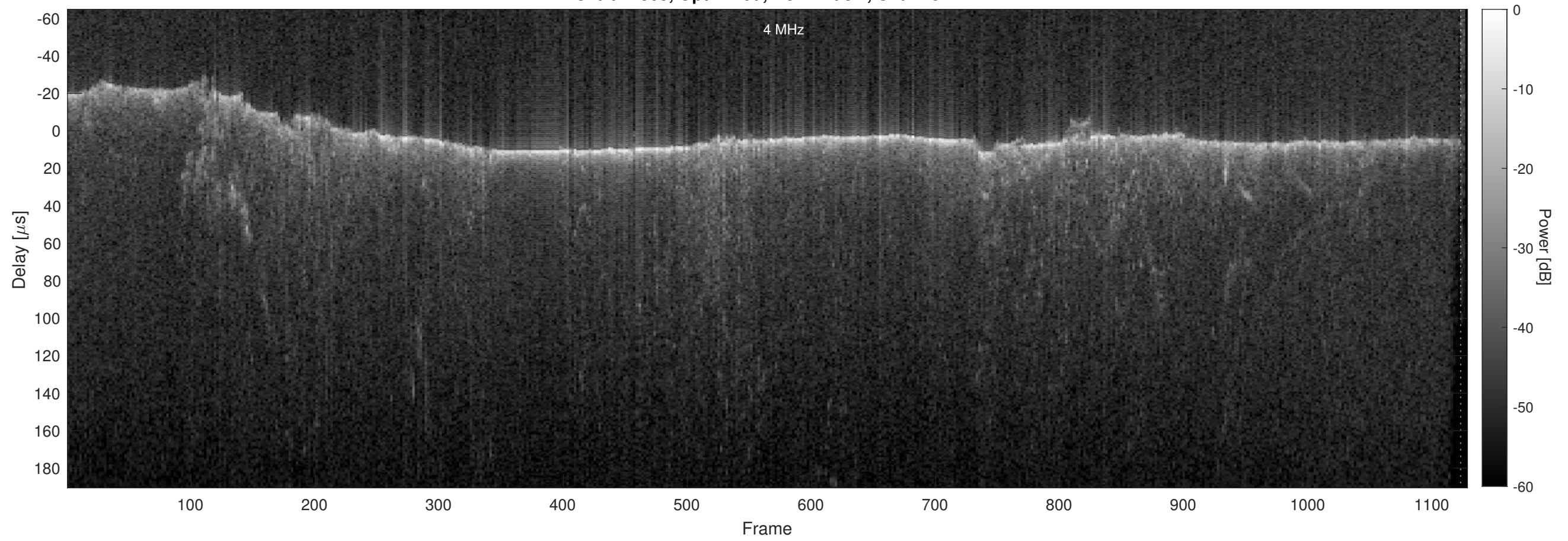
Orbit 12305, Optimized, No Window, Channel 2
