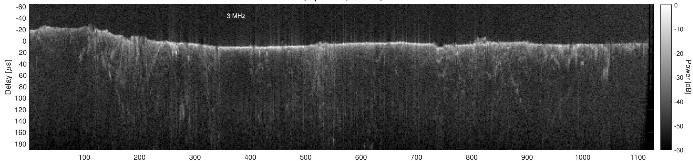
Orbit 12305, Cluttergram
