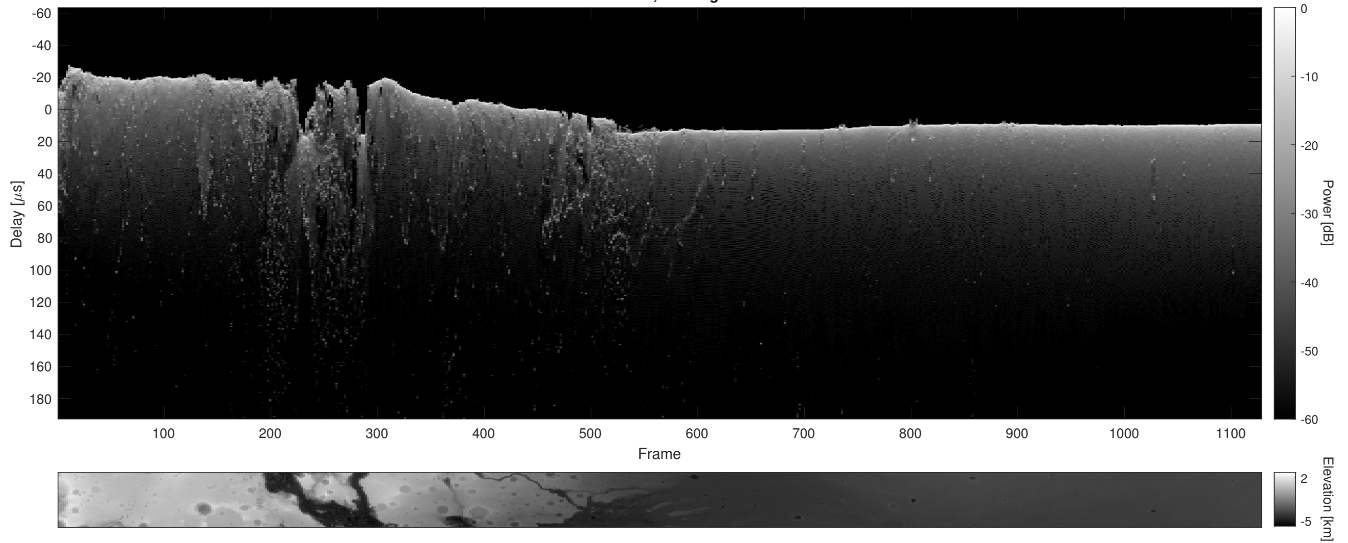
Orbit 12307, Cluttergram
