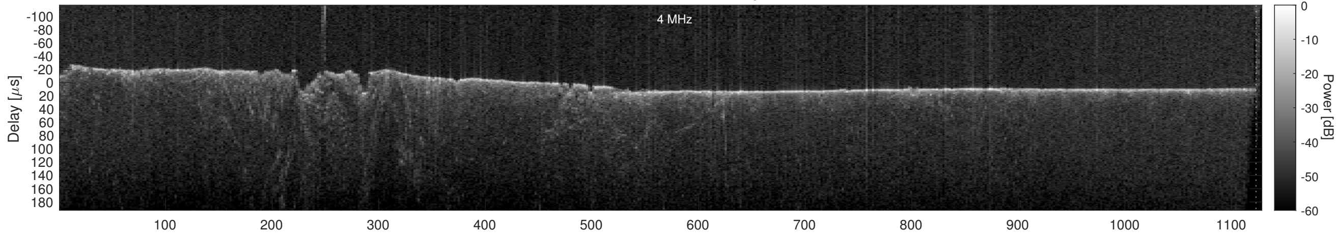
Orbit 12307, Cluttergram
