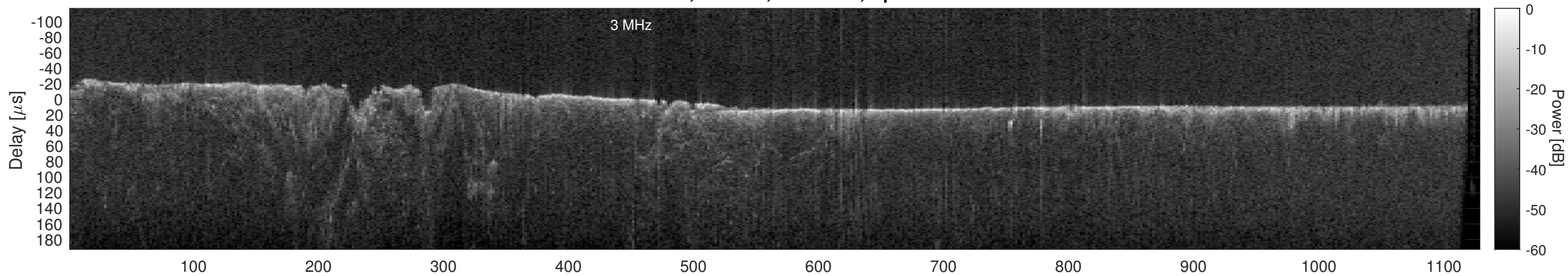
Orbit 12307, Cluttergram
