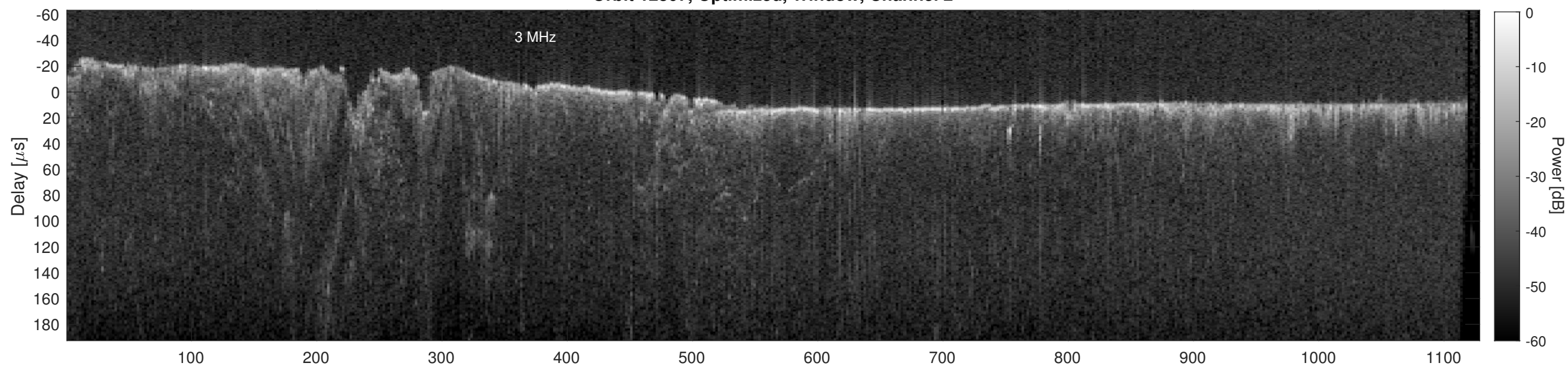
Orbit 12307, Cluttergram
