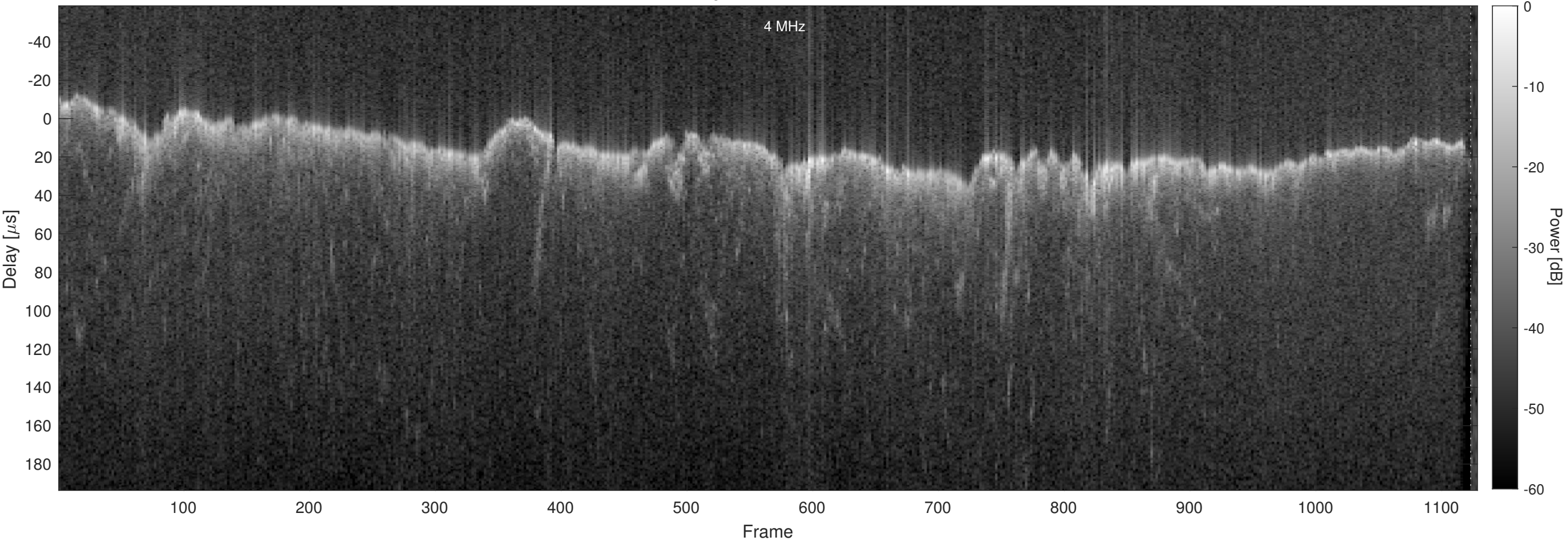
Orbit 12310, Chapman, No Window, Channel 2
