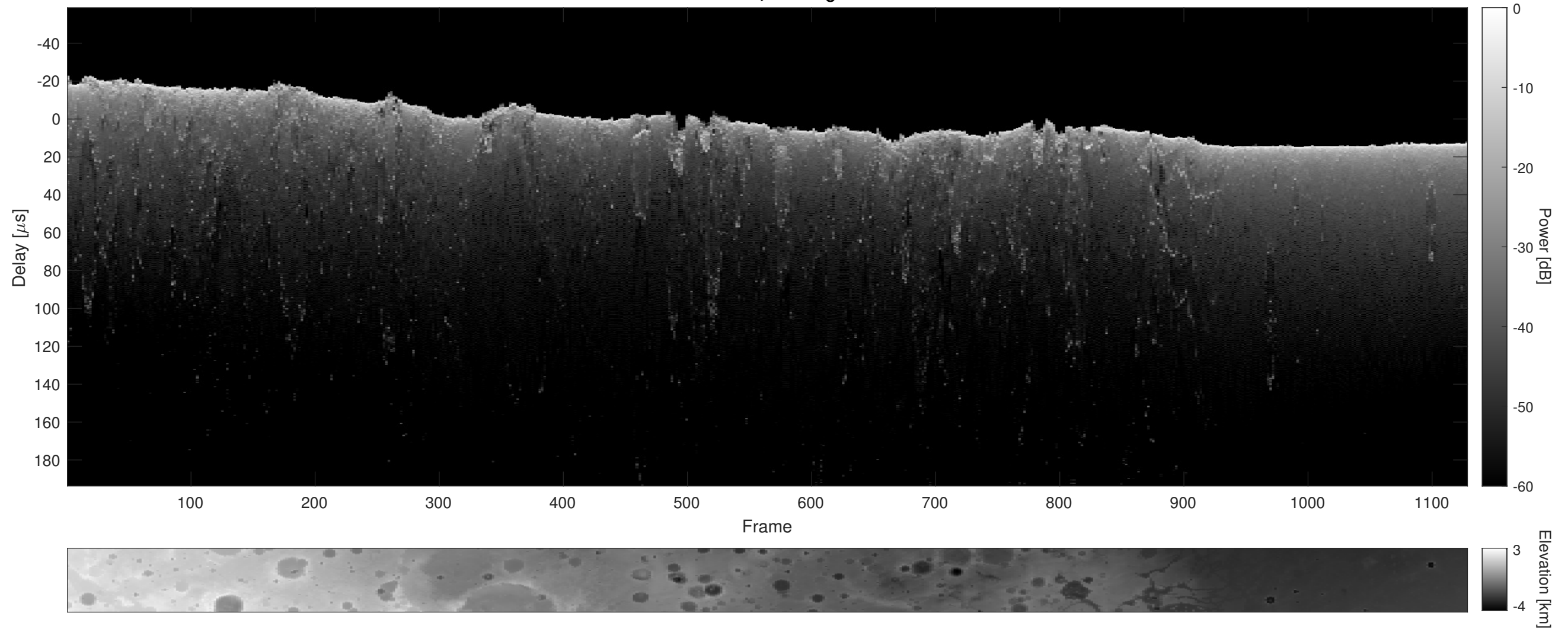
Orbit 12310, Cluttergram
