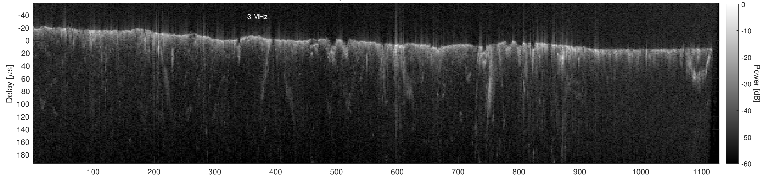
Orbit 12310, Cluttergram
