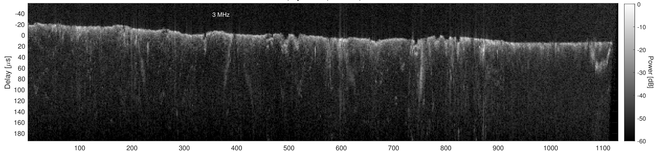
Orbit 12310, Cluttergram
