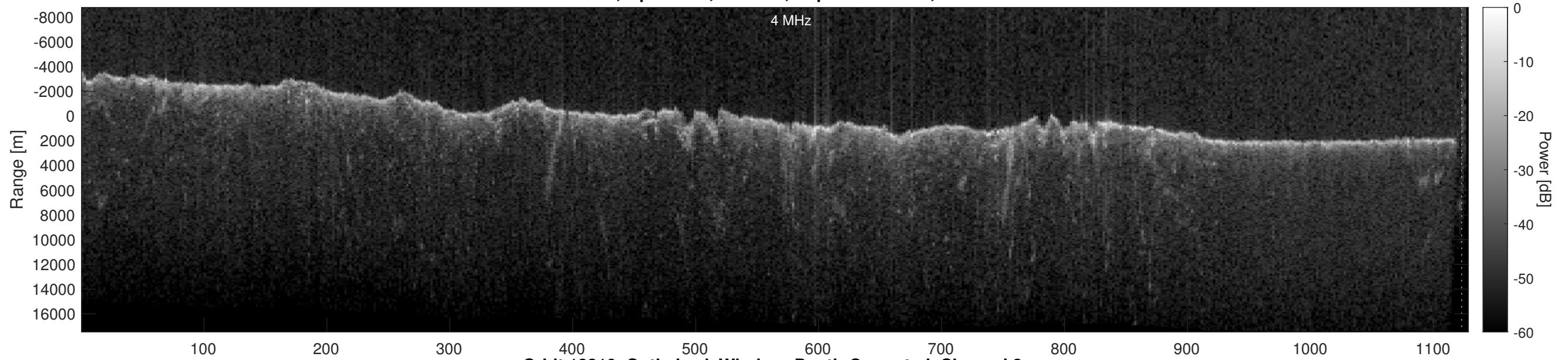
Orbit 12310, Optimized, Window, Depth-Corrected, Channel 2
