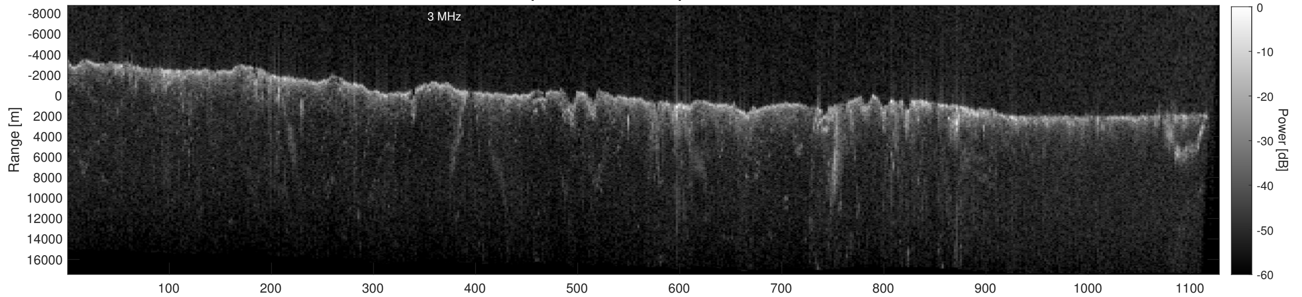
Orbit 12310, Depth-Corrected Cluttergram
