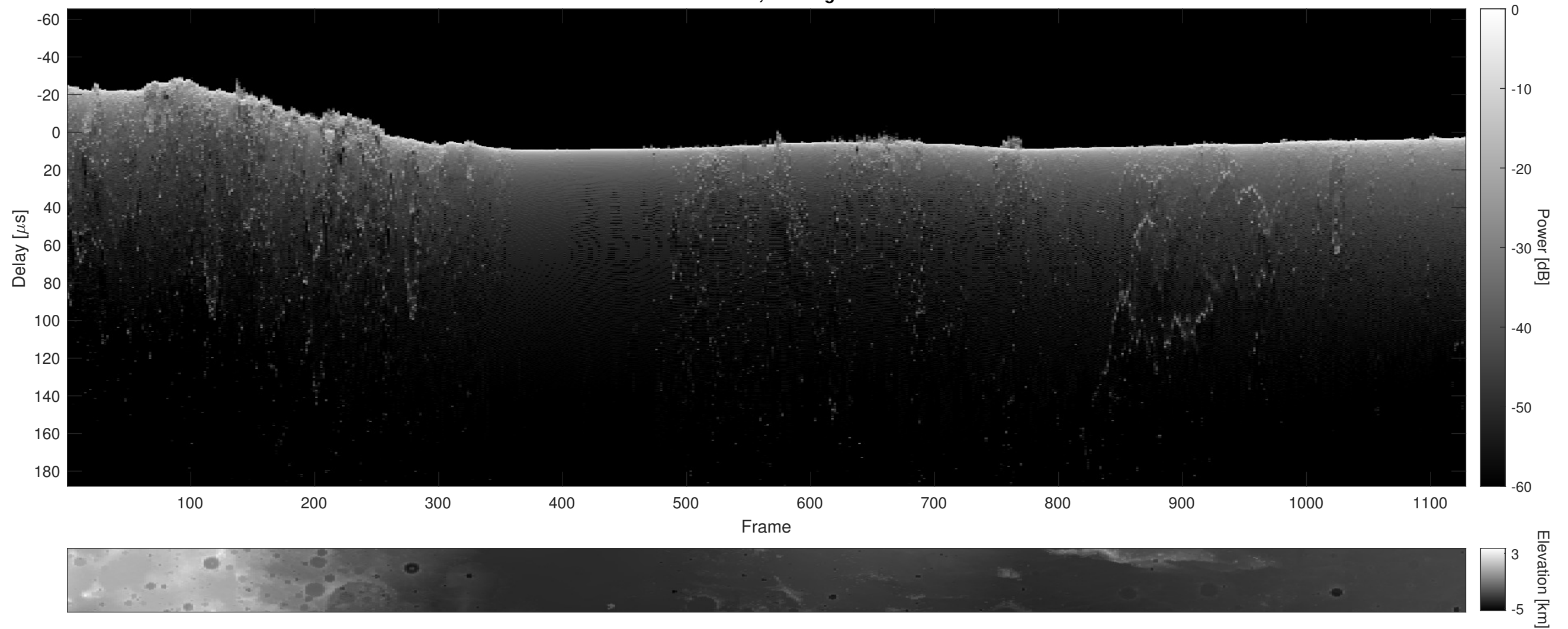
Orbit 12312, Cluttergram
