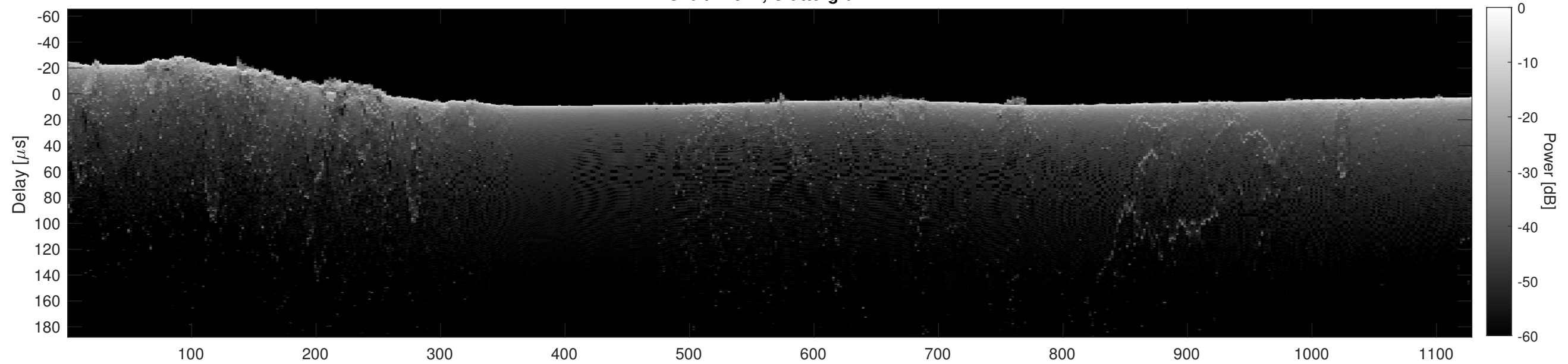
Orbit 12312, Cluttergram
