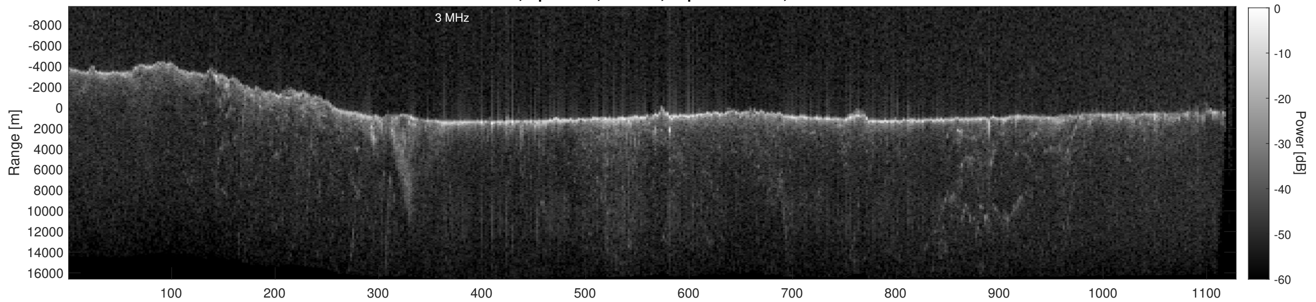
Orbit 12312, Depth-Corrected Cluttergram
