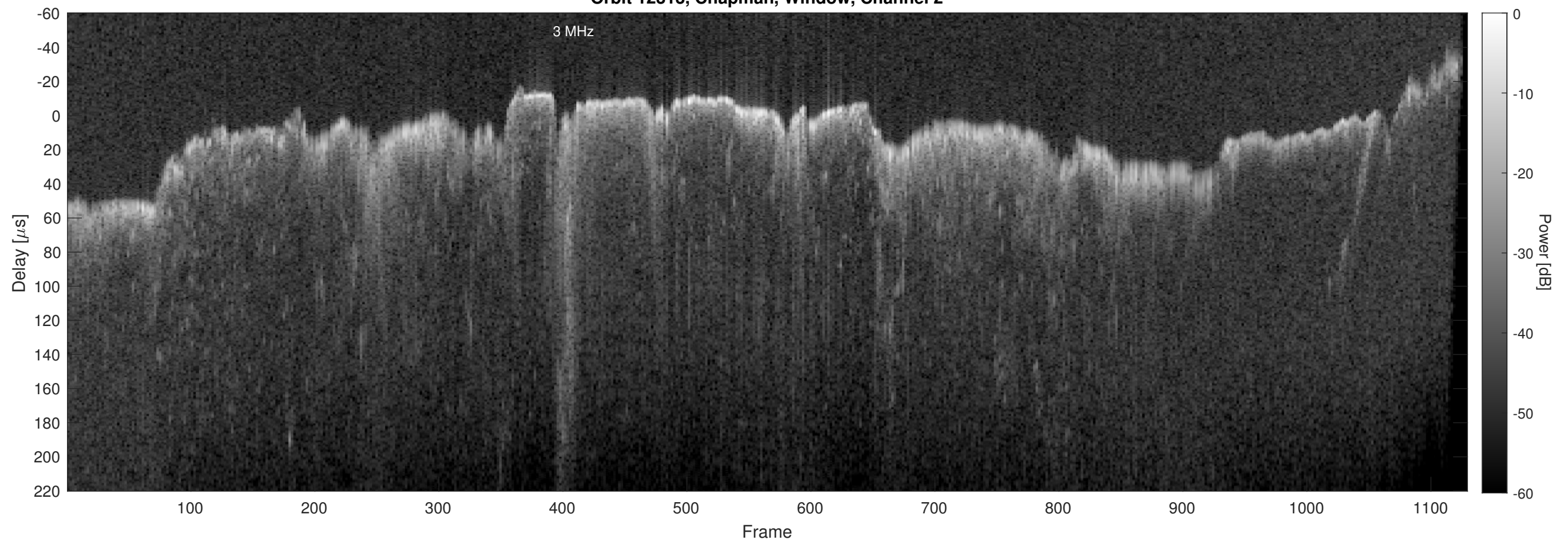
Orbit 12313, Chapman, Window, Channel 2
