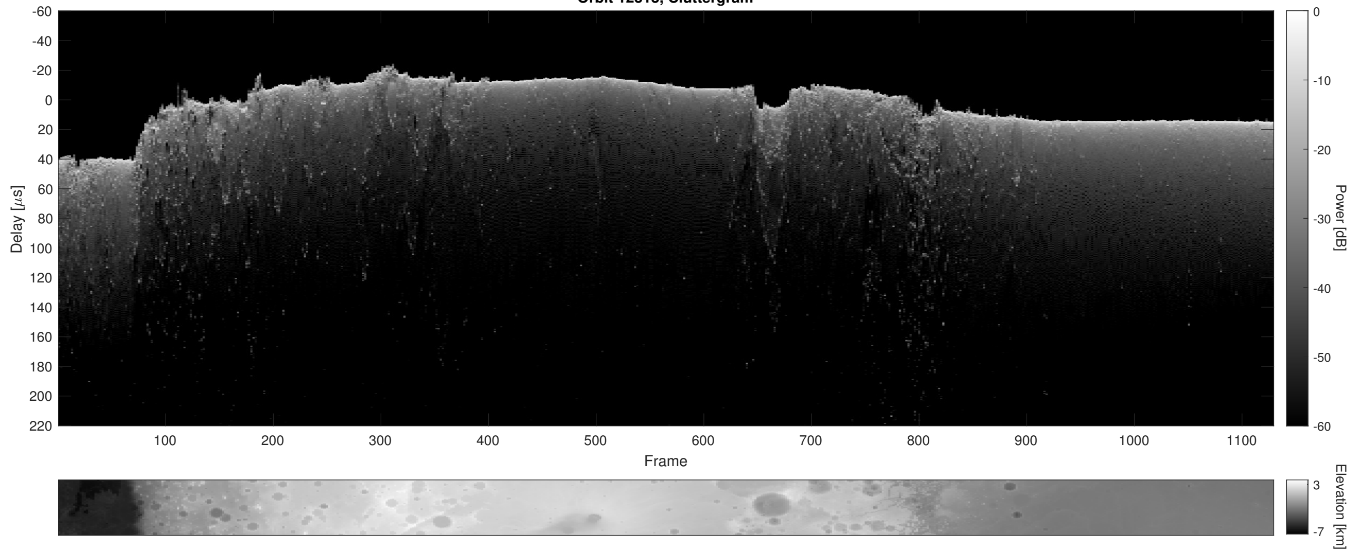
Orbit 12313, Cluttergram
