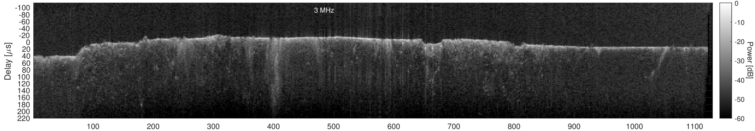
Orbit 12313, Cluttergram
