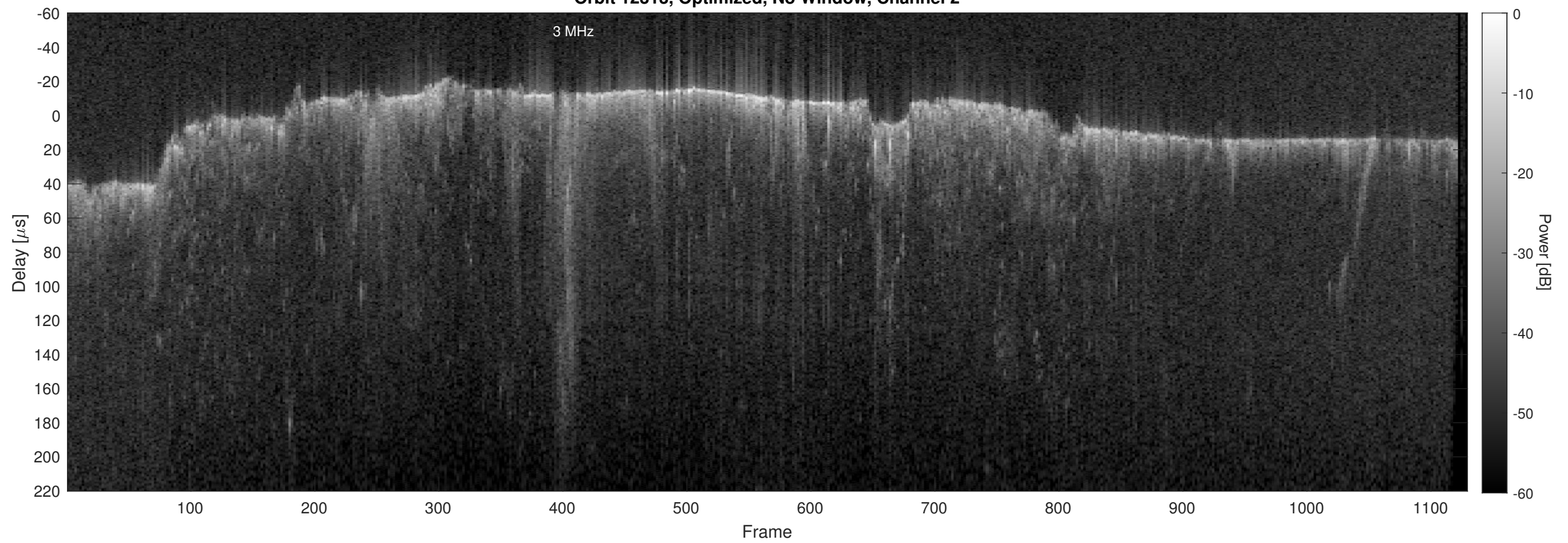
Orbit 12313, Optimized, No Window, Channel 2
