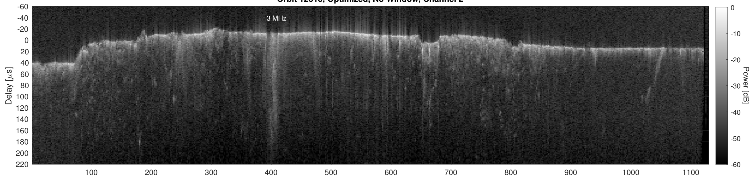
Orbit 12313, Cluttergram
