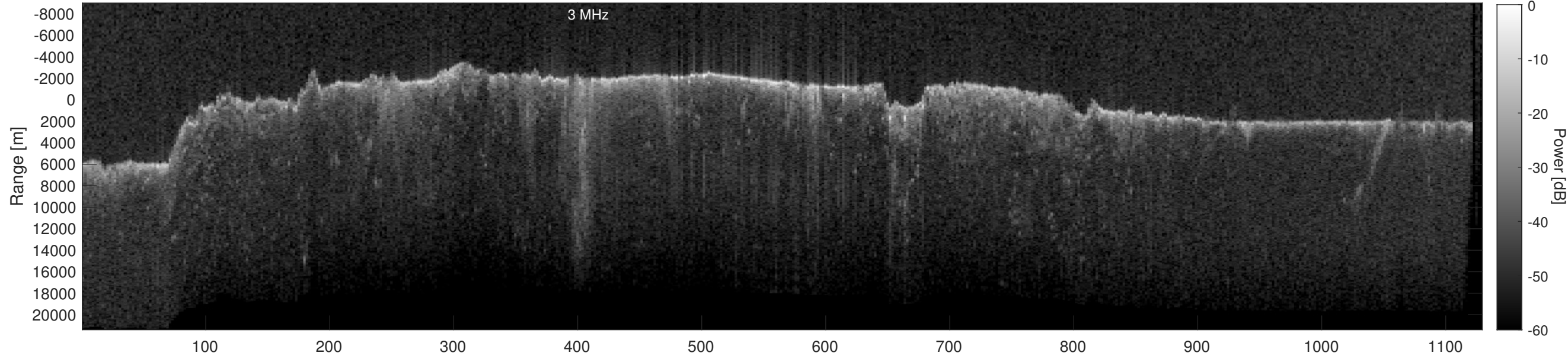
Orbit 12313, Depth-Corrected Cluttergram
