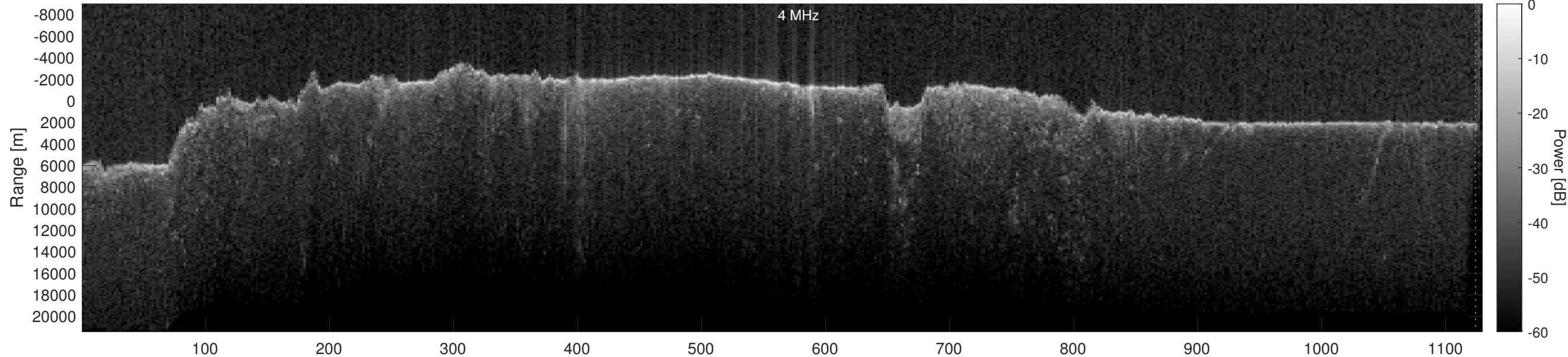
Orbit 12313, Optimized, Window, Depth-Corrected, Channel 2
