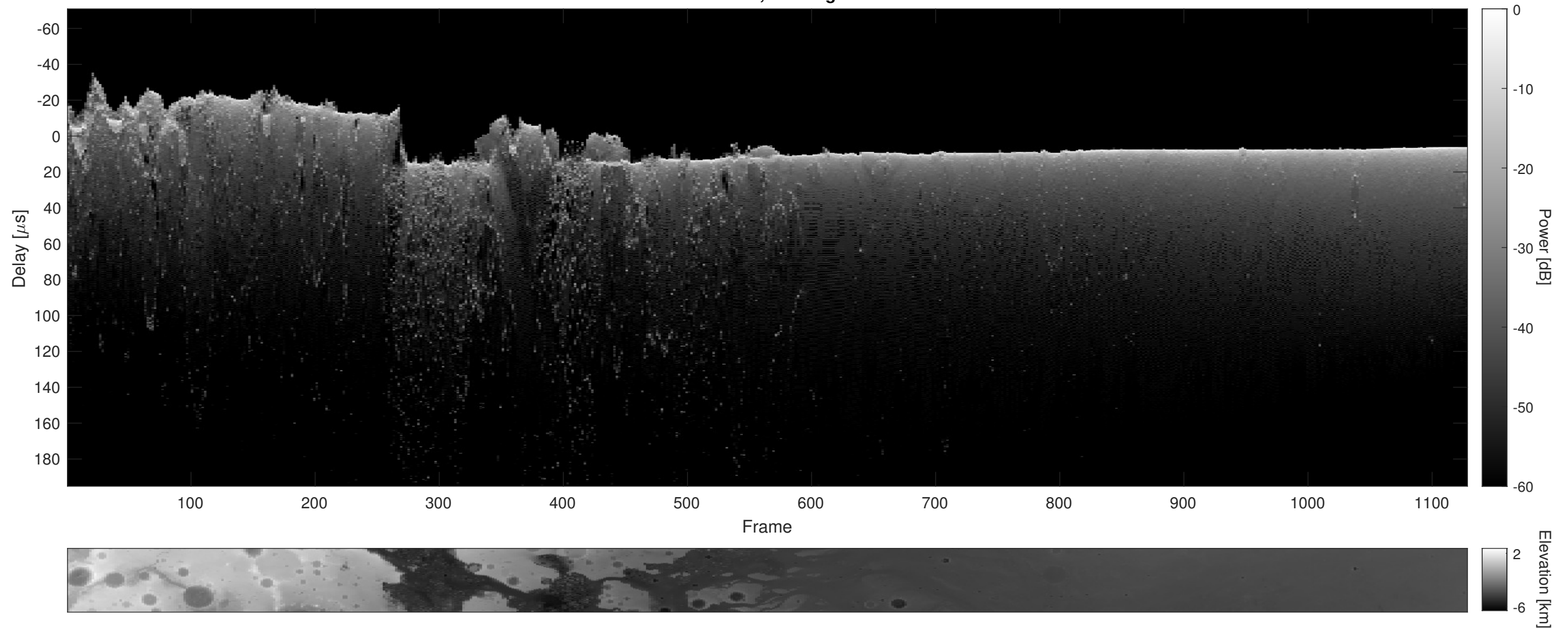
Orbit 12314, Cluttergram
