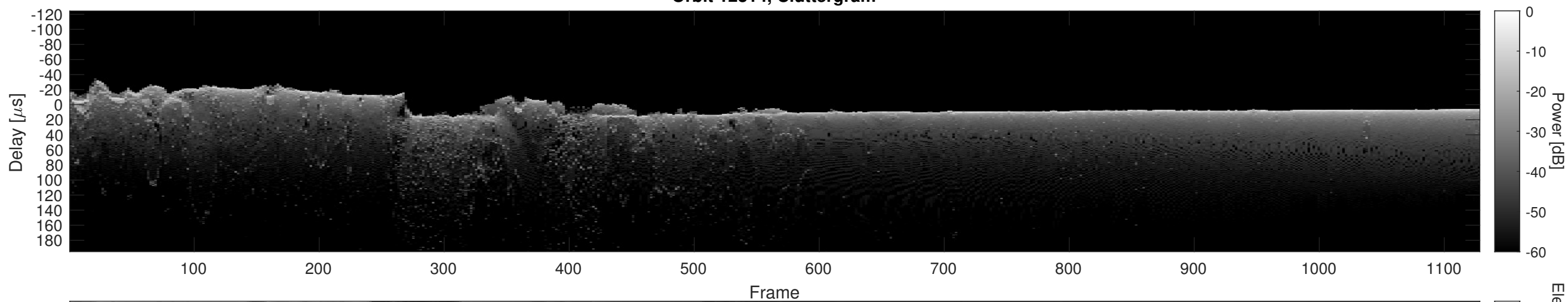
Orbit 12314, Cluttergram
