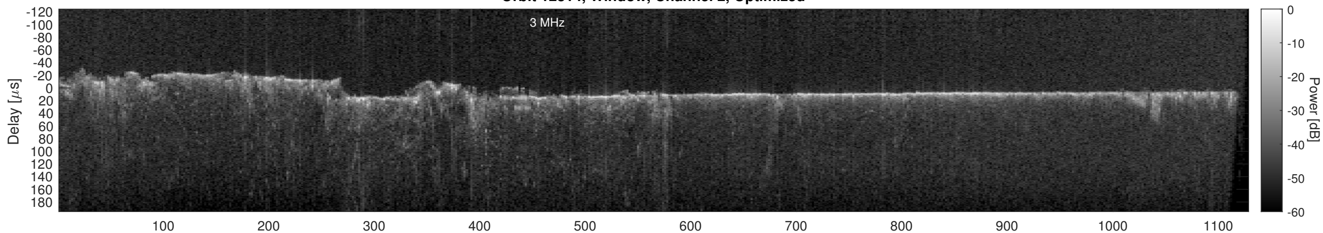
Orbit 12314, Cluttergram
