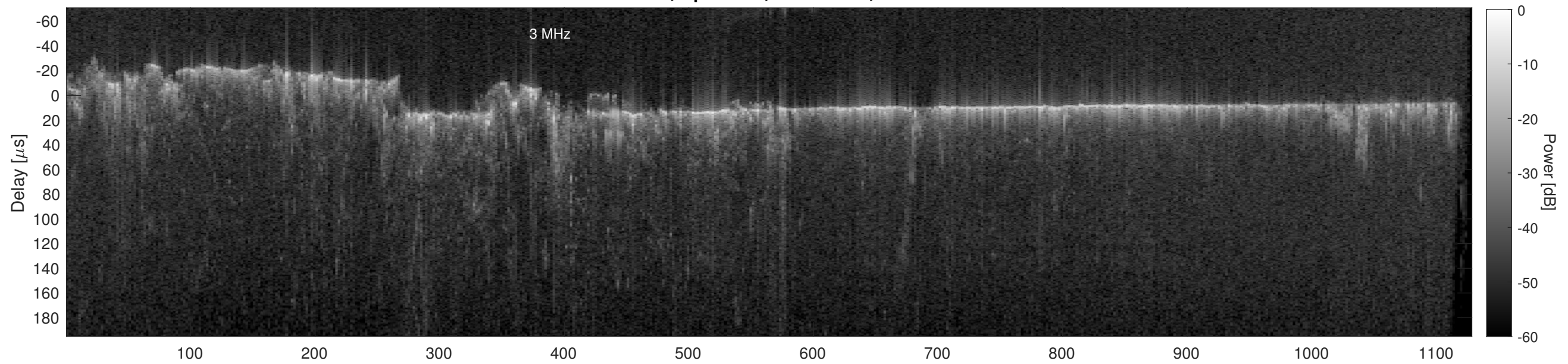
Orbit 12314, Cluttergram
