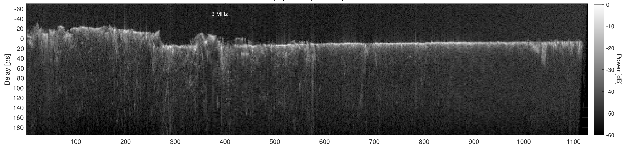
Orbit 12314, Cluttergram
