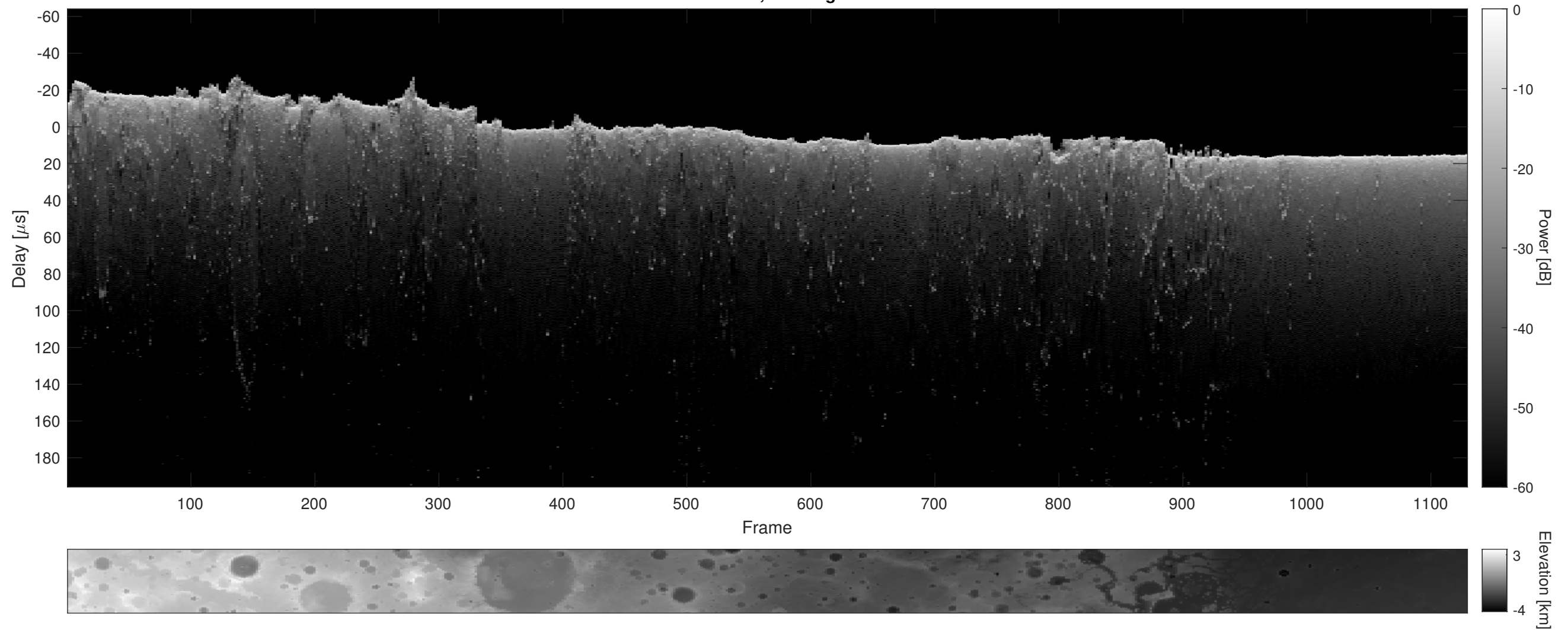
Orbit 12317, Cluttergram
