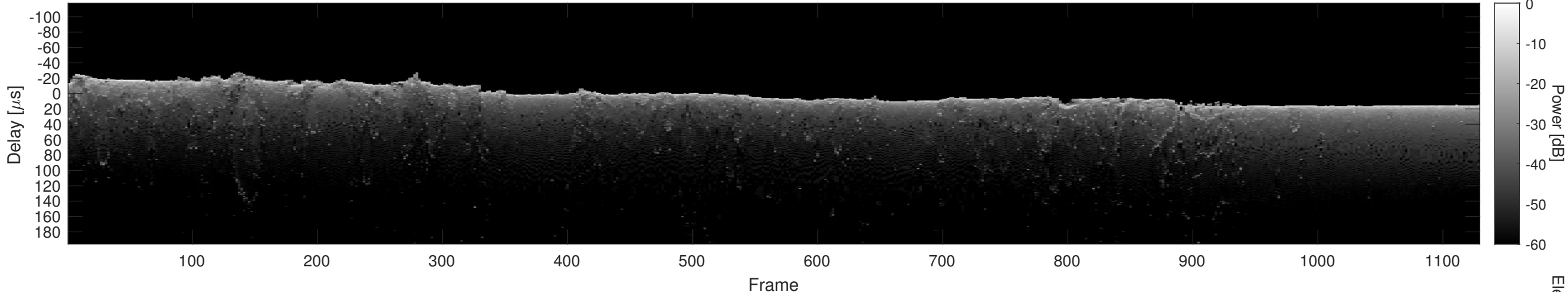
Orbit 12317, Cluttergram
