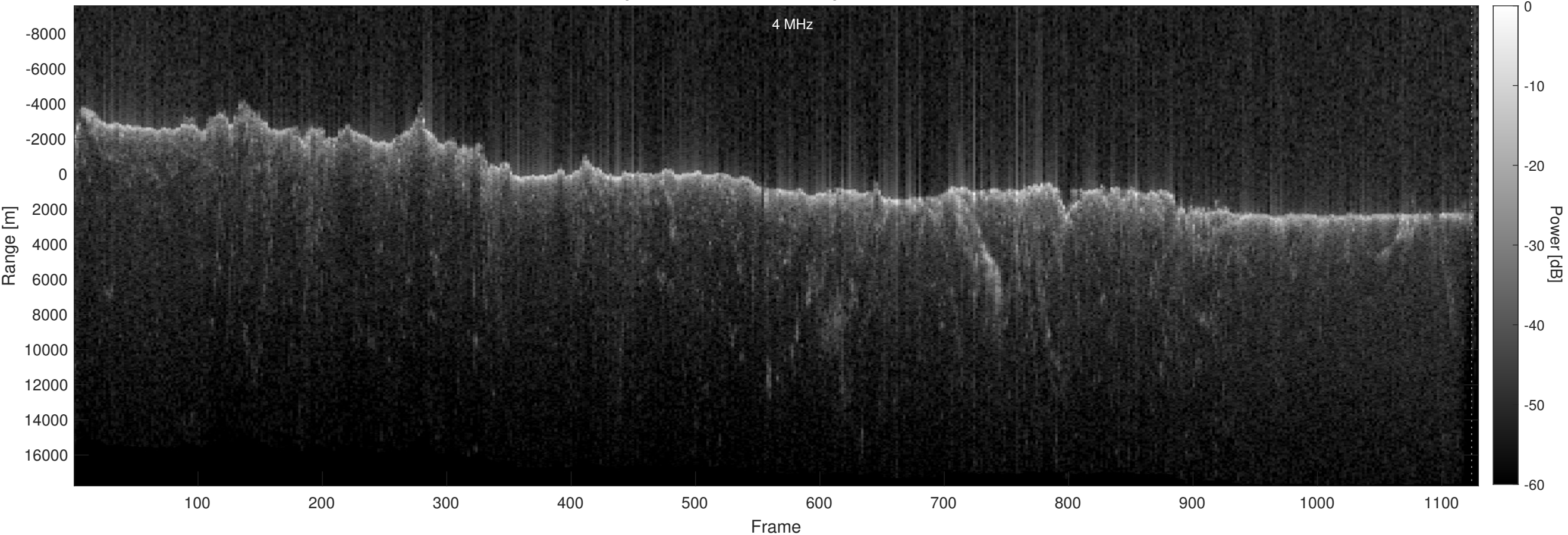
Orbit 12317, Optimized, No Window, Depth-Corrected, Channel 2
