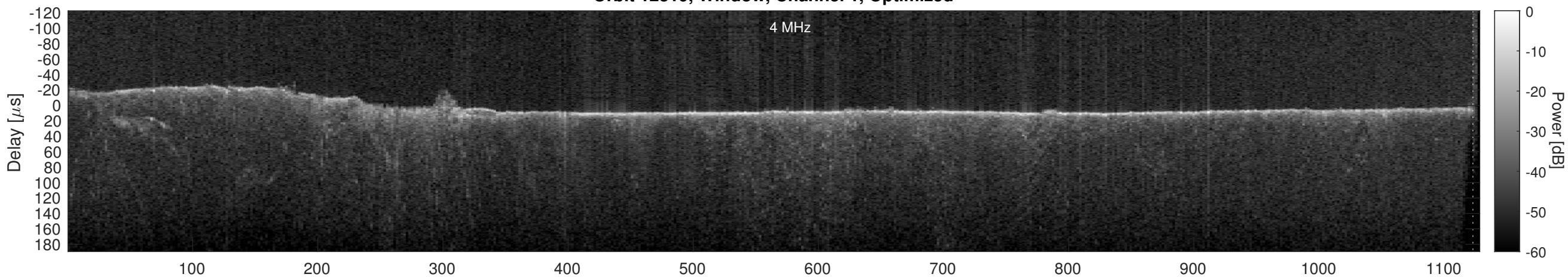
Orbit 12319, Cluttergram
